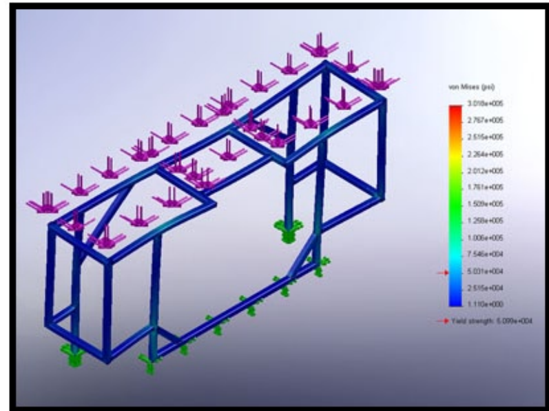
3-D analysis of a modular frame using CosmosWorks 3-D analysis software.
